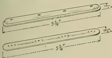
Fig. 141.—Types of Roofing "Cleats."
